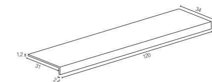
GRADINO PLUS BORDO* 34x120x4,5 cm Rect - 13 3/8 "x48"x1 3/4 " LUX ± 9,5 mm
