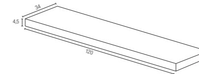
GRADINO PLUS ANGOLARE DX* 34x120x4,5 cm Rect - 13 3/8 "x48"x1 3/4 " SOFT ± 9,5 mm
